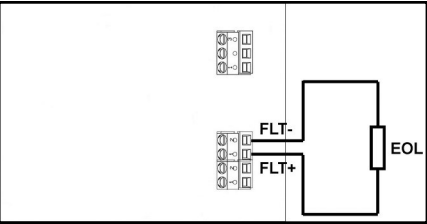
Picture 8 - Wiring example for the FLT port
