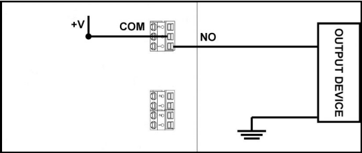
Picture 7 - Wiring example for relay switch output
